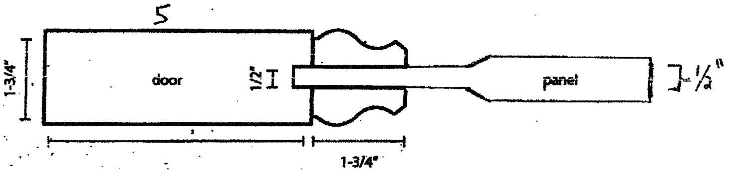
panel detail overhead
