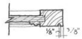
DETAIL 3/4" = 1'-0"
