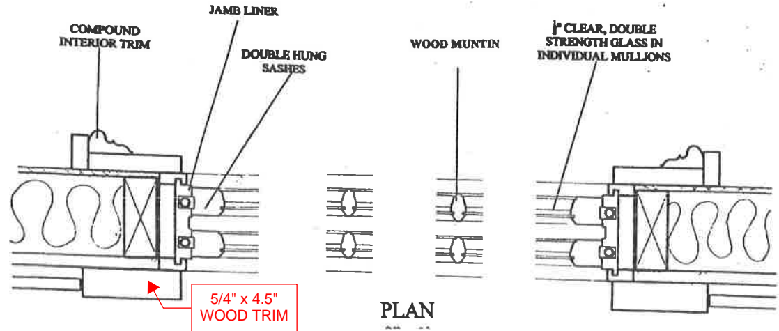
SECTION 3" = 1'
