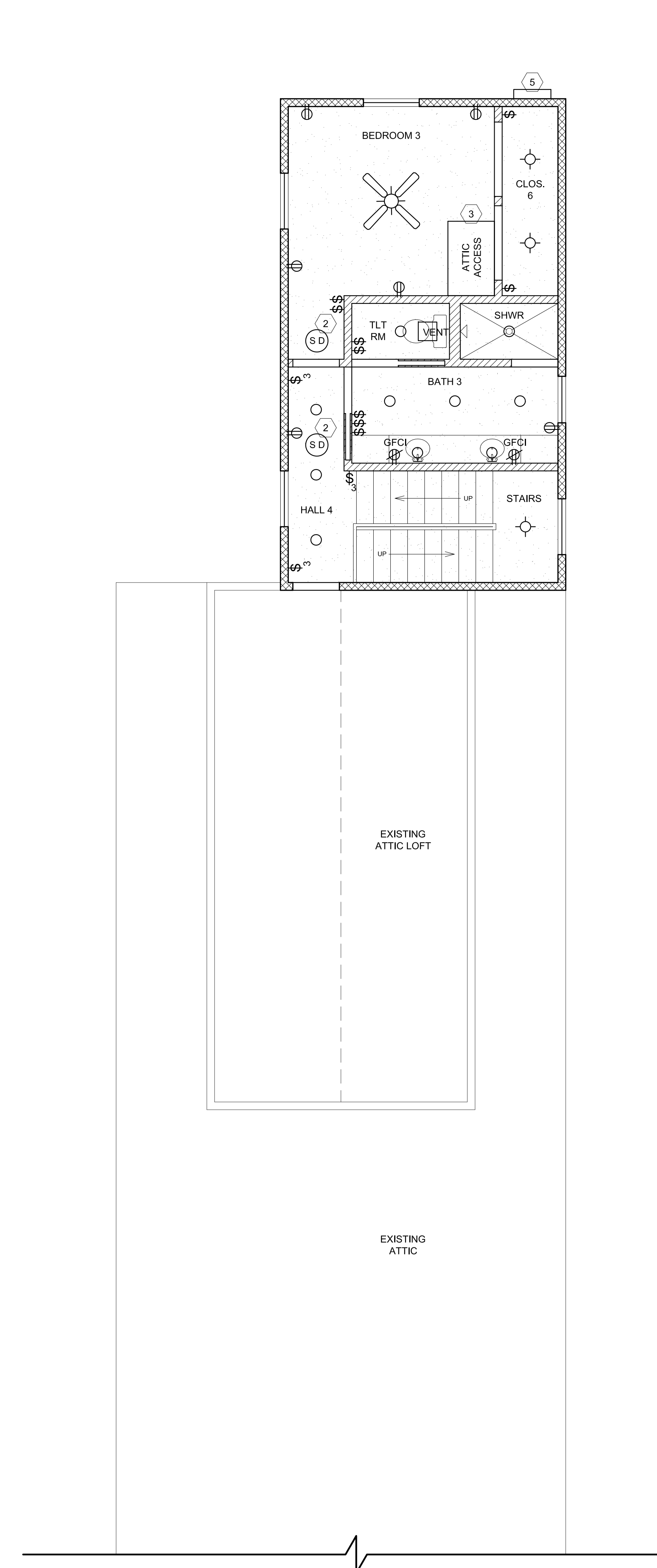
PROPOSED SECOND FLOOR REFLECTED CLG PLAN SCALE: 1/4" = 1'-0"
