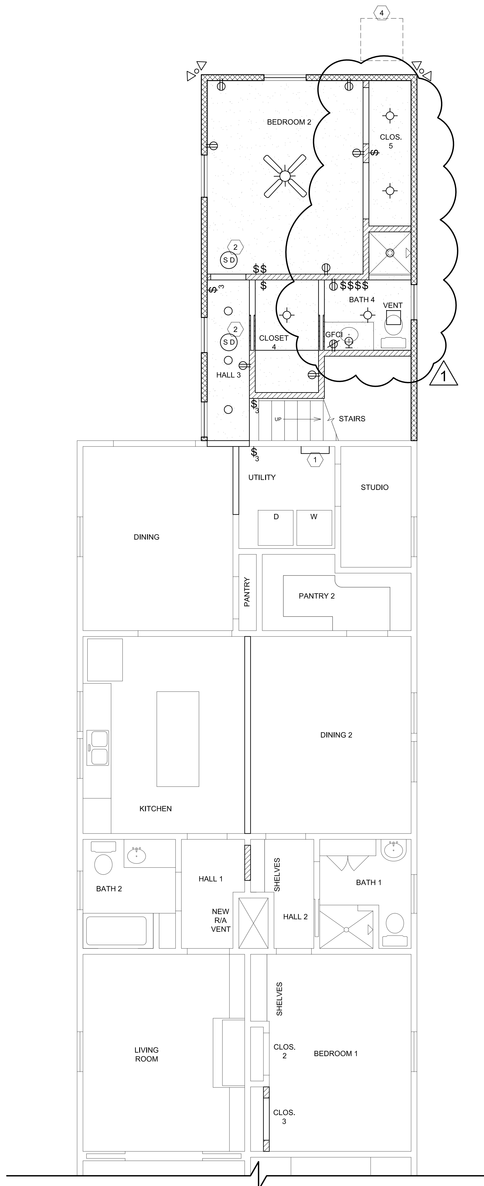
PROPOSED FIRST FLOOR REFLECTED CLG PLAN SCALE: 1/4" = 1'-0"
