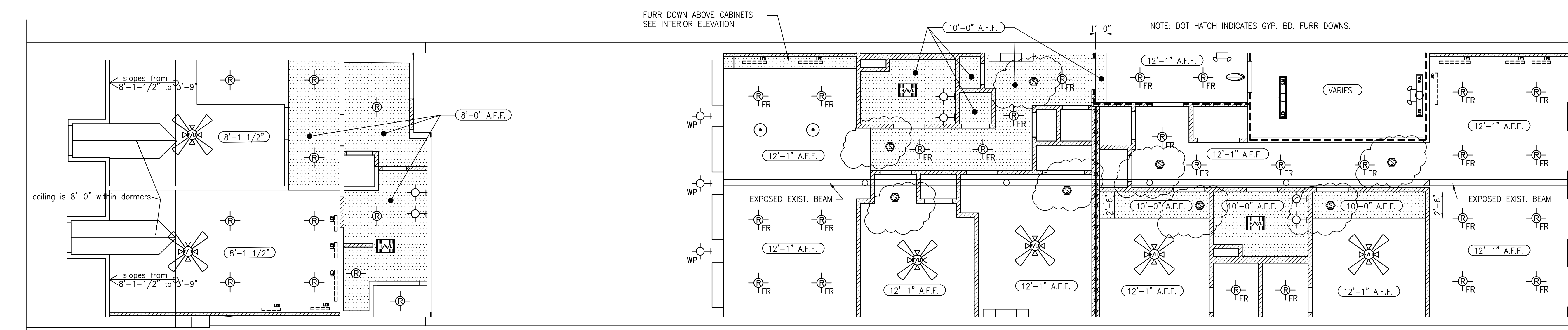
1 NEW FIRST FLOOR REFLECTED CEILING PLAN SCALE: 3/16"=1'-0"
