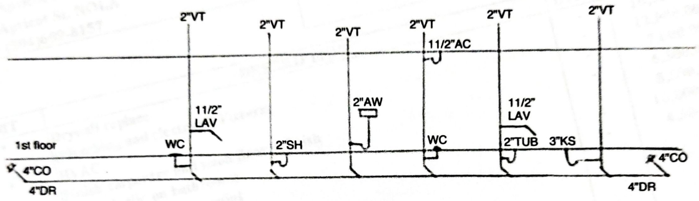
SEWER DIGRAM 8610 APRICOT STREET
