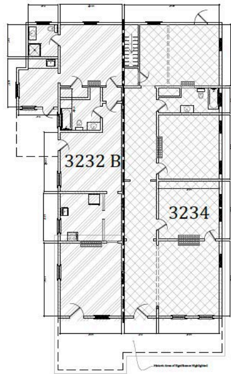
Existing Second Level Units Scale: 1/8" = 1'-0"
