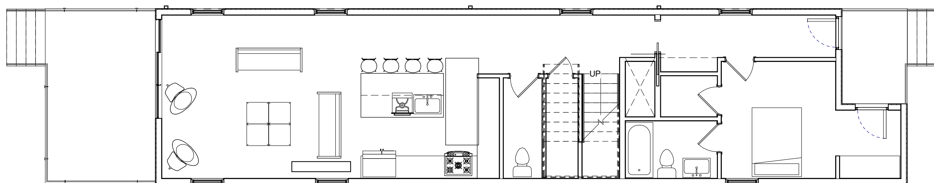
2 Floor Plan - Level 1 3/16" = 1'-0"
