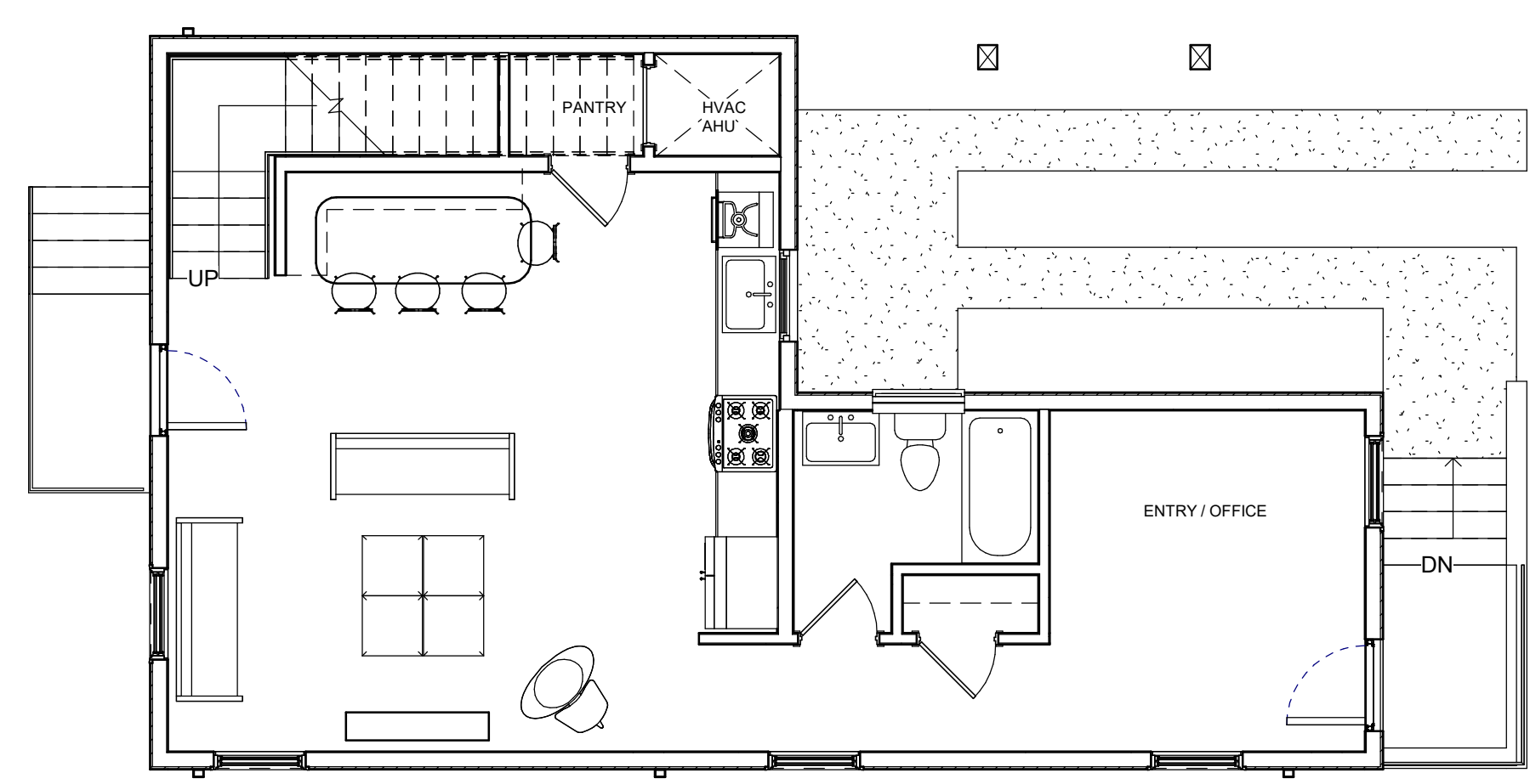
2 Level 1 3/16" = 1'-0"
