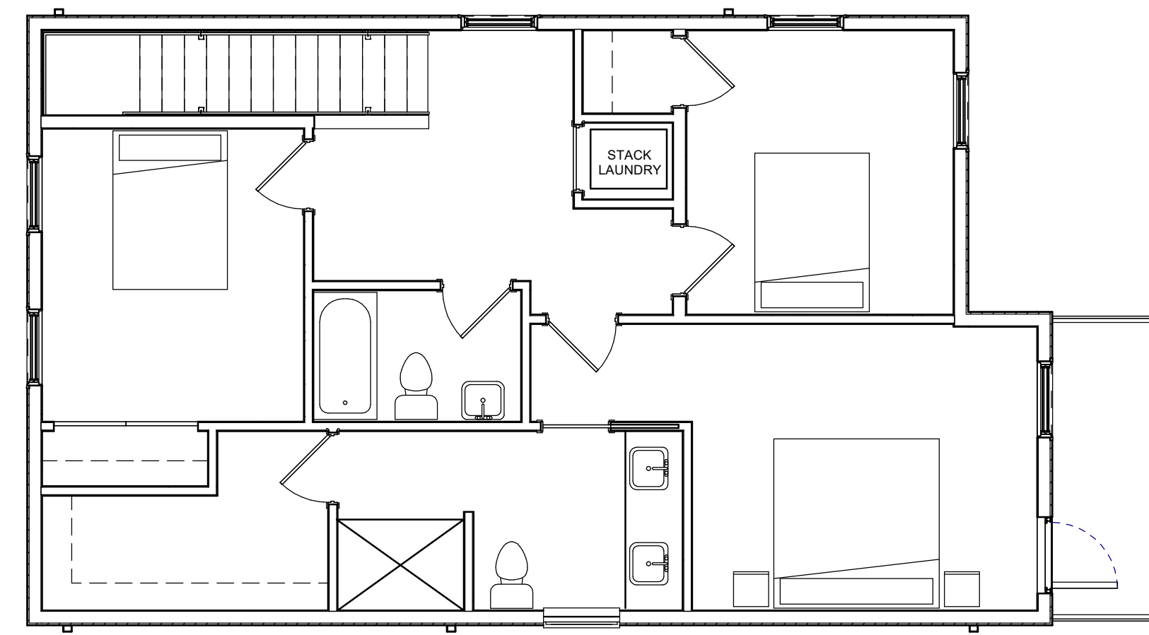
3 Level 2 3/16" = 1'-0"
