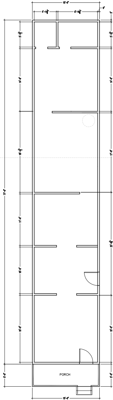
Existing First Floor
